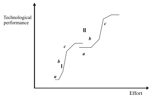
Figure 2. Technological S-Curve
